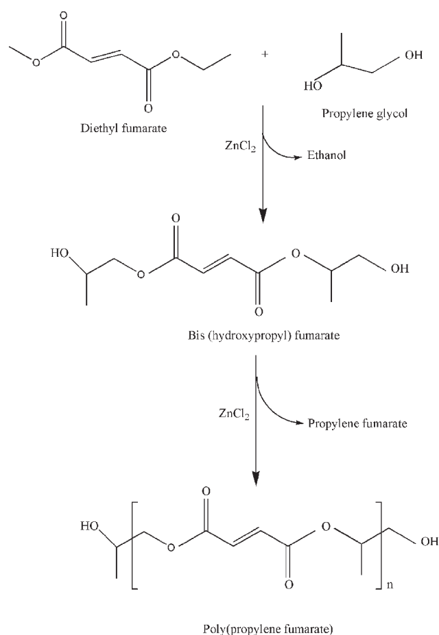
Figure 1. Reaction scheme for the step polymerization of poly (propylene fumarate) from propylene glycol and diethyl fumarate.
