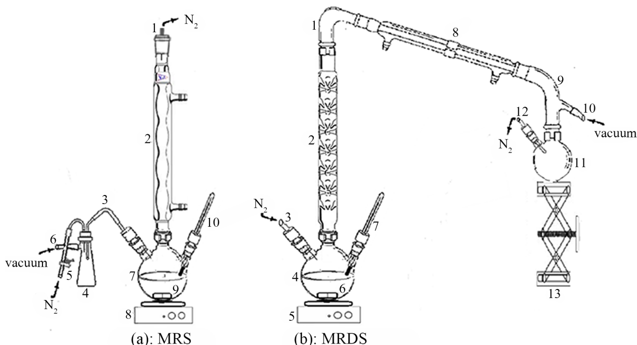
Figure 2. (a): Modified reflux system (MRS). (b): Mixed reflux-distillation system (MRDS).
