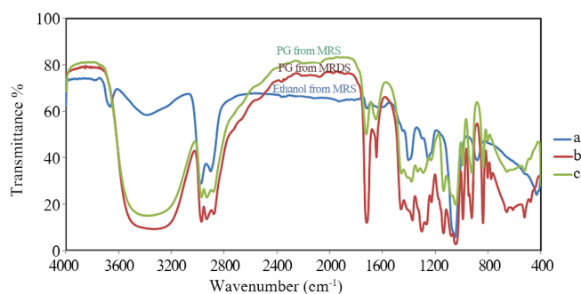
Figure 3. (a): FTIR of ethanol (as a by-product): sampling from the vapor phase of the reactor in MRS. (b): FTIR of propylene glycol (as a by-product) from MRDS. (c): FTIR of propylene glycol (as a by-product) from MRS.
