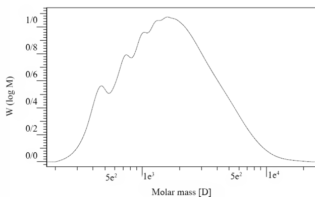
Figure 7. GPC chromatogram of final PPF
